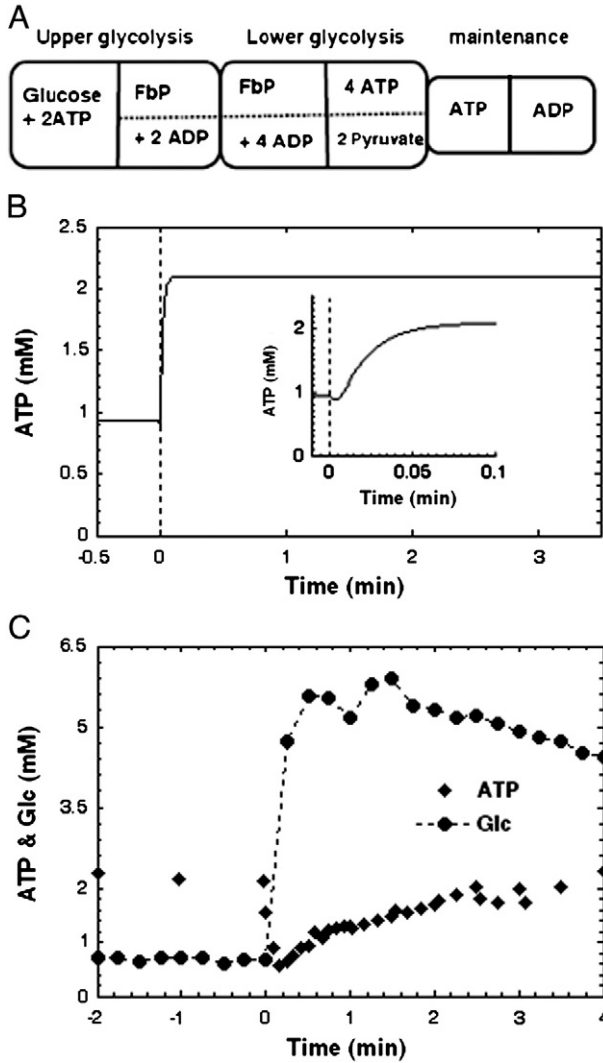
Fig. 1. (A): The domino of glycolysis split into two consecutive dominoes, i.e., upper glycolysis leading from glucose to fructose-1,6-bisphosphate (FbP) and lower glycolysis from FbP to pyruvate and 4ATPs and then further from pyruvate to ethanol and carbon dioxide (see Materials and Methods). Glycolysis leads to the net production of two ATPs. On the right: the maintenance domino that persists. (B): Model calculations of ATP dynamics based on second domino scheme under glucose limited and excess conditions. Vertical dotted line indicates separation of glucose limited and rich conditions. (C): ‘ATP paradox’ observed in S. cerevisiae growing in glucose limited continuous anaerobic culture ( D = 0.1 \text{ h}^{-1} with steady state C_{\text{glc}} = 0.67 \text{ mM} ). After sudden addition of extra glucose (i.e. glucose increase to C_{\text{glc}} = 5.56 \text{ mM} ) at t = 0 the intracellular concentration of ATP rapidly and significantly decreases and recovers in 4 min, and only partly.
